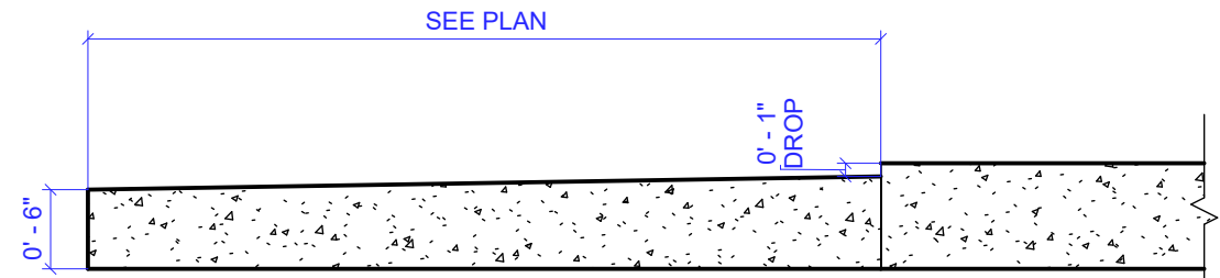
2 TYPICAL SECTION AT BALCONIES DM-04 N.T.S
