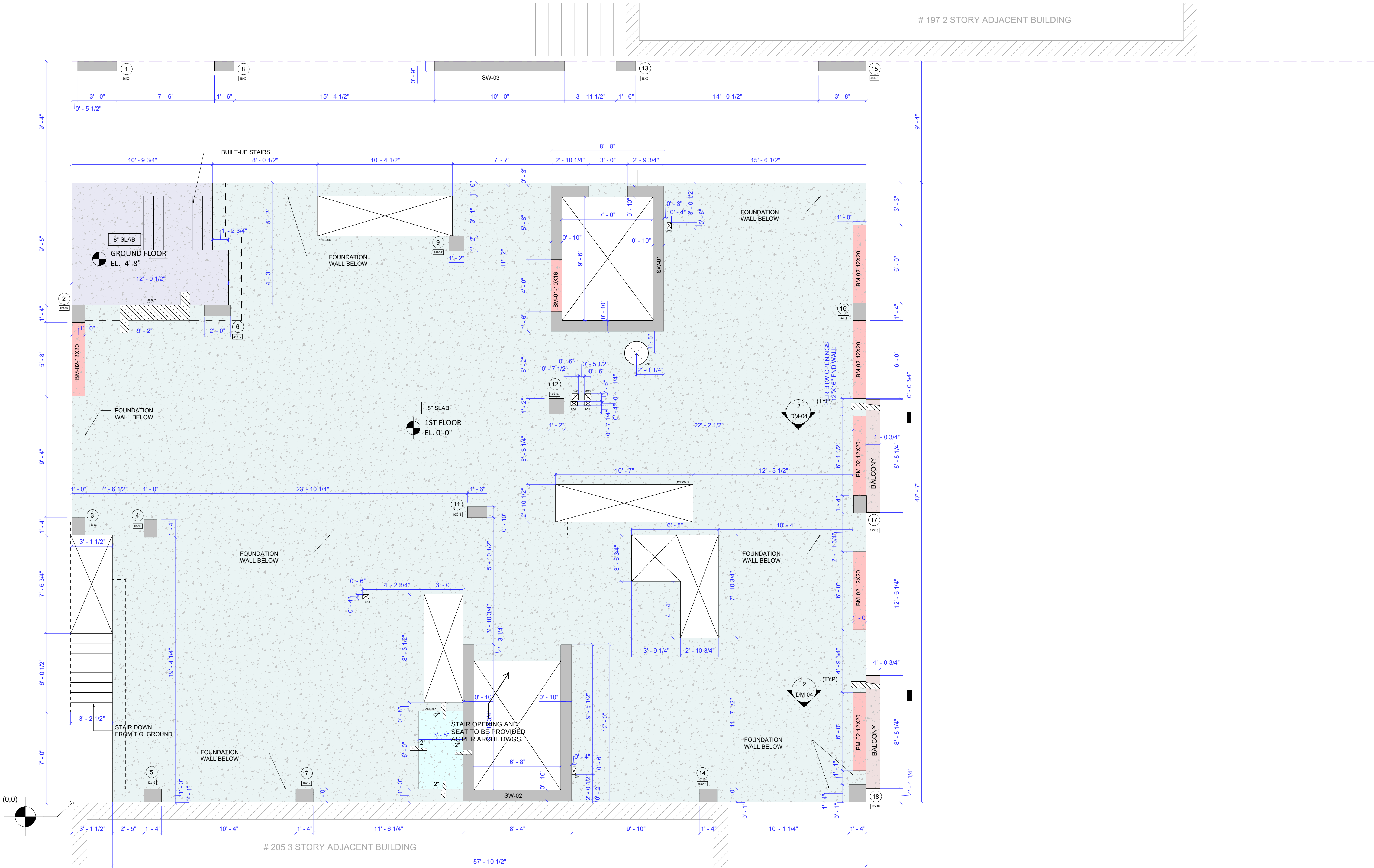
1 1ST FLOOR DIMENSION PLAN 1/4" = 1'-0"
